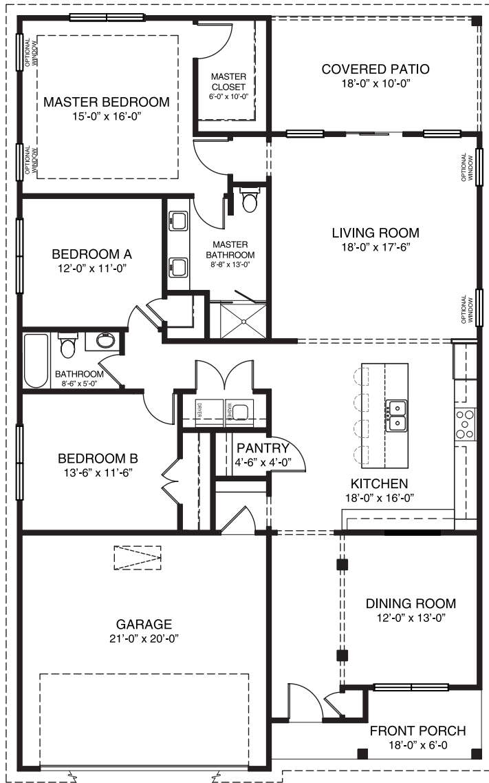
FLOOR PLAN
